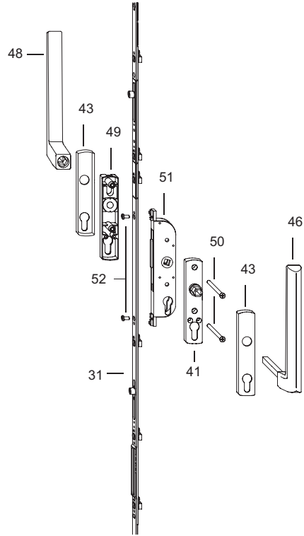
Manilla interior y exterior cerrable Manilla exterior normal
